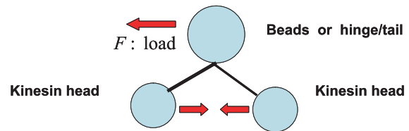
Figure 1: A model of double-headed motor, kinesin.
