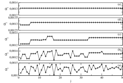
Figure 2: The evolution of observed frequencies \Omega_j (4) for different couplings (a) d = 0 , (b) d = 0.0005 , (c) d = 0.001 , (d) d = 0.0015 , and (e) d = 0.0025 . \varepsilon = 0.0000001 , \Delta\varepsilon = 0.0000001 , and N = 50
