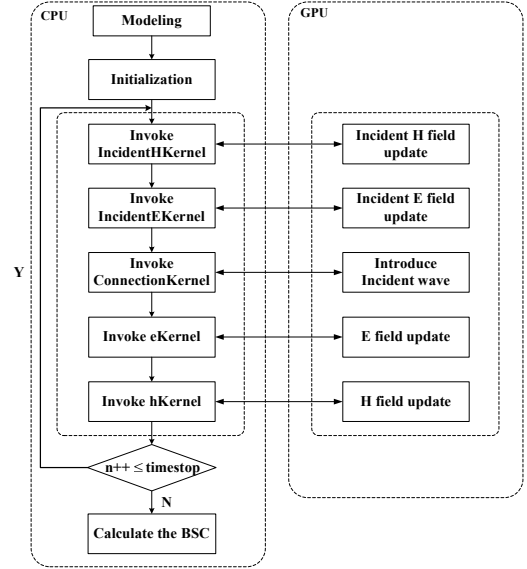
Fig. 5. The flowchart of GPU based FDTD algorithm for rough surface
