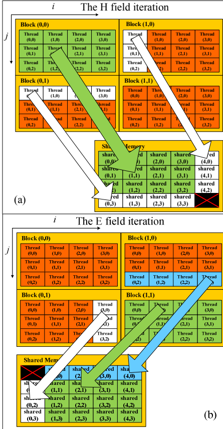
Fig. 4. Data transfers from global memory to shared memory
