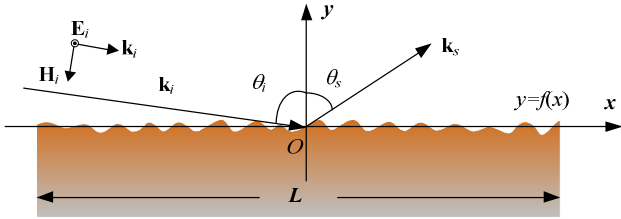
Fig. 1. Geometry for EM scattering from 1-D rough surface (TM wave).
