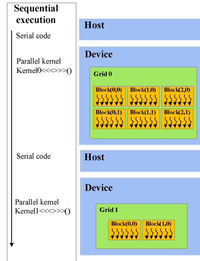
Fig. 3. The CUDA programming model [11]
