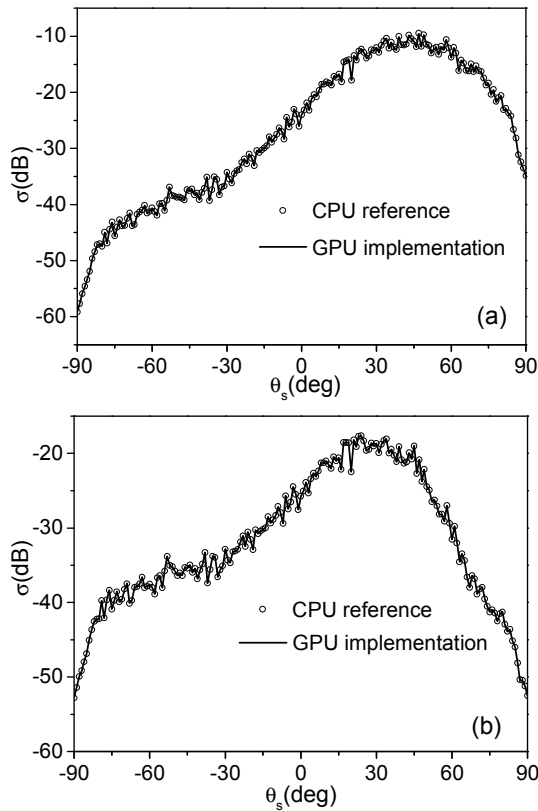
Fig. 6. Comparisons of the bistatic scattering from a soil surface by two implementations: (a) TM case; (b) TE case.
