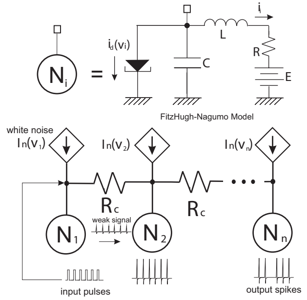
Figure 3: Block diagram of serially-connected circuits with noise-assisted spike propagation
