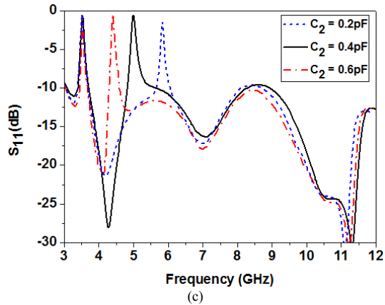
Figure 2. (a) Geometry of the UWB antenna with controllable band notches. (b) Effect of varactor diodes capacitance C_1 and (c) C_2 on return loss.
