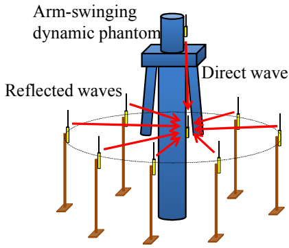
Fig. 2 Configuration of the BAN fading emulator
