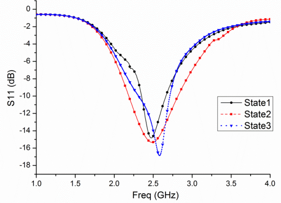
Fig. 2. Simulated S_{11} for the three different operating modes.
