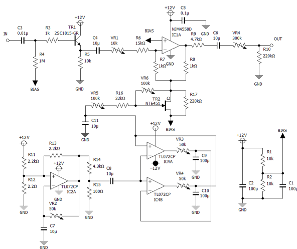
Figure 13: Circuit implementation of the system that append chaotic fluctuation.
