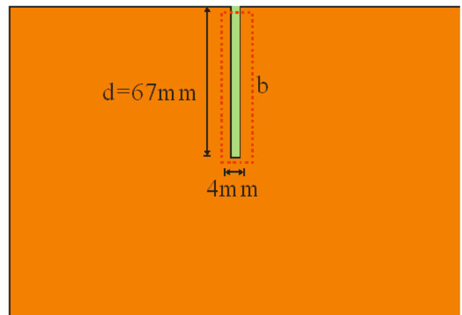
Figure.2 Antenna body.
