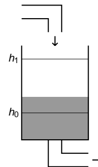
Figure 1: A schematic diagram of the water tank system. The tank has a controllable incoming flow and a constant outgoing flow.
