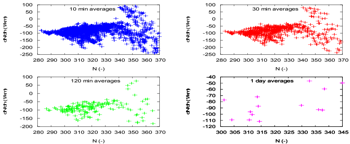
Fig. 6 Dependence of vertical gradient of refractivity in heights between 126 m and 12 m on ground refractivity in 12 m
