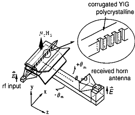
Fig.1 experimental setup
