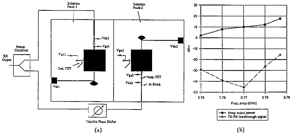
Figure 1: (a) Sequentially rotated two element active array (b) Array output power and transmit-receive feedthrough signal
