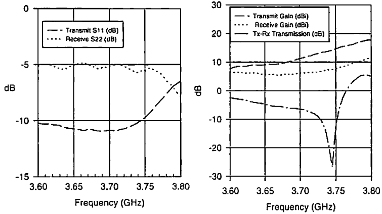
Figure 3 : Measured S-parameters, transmit and receive gains for an active circulator antenna
