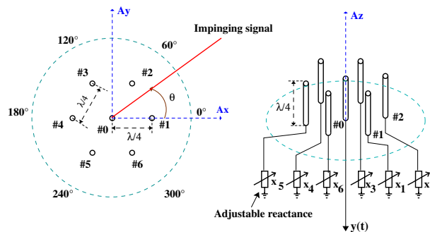
Figure 1: 7-element ESPAR antenna schemes
