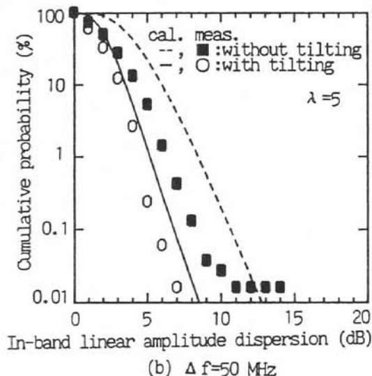
Fig.4 Cumulative distribution of in-band linear amplitude dispersion.
