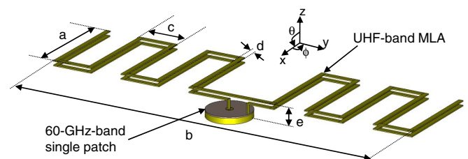
Fig. 1. Proposed antenna for UHF- and 60-GHz bands with single feed structure.
