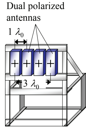
Figure 2: Geometry of base station antenna.
