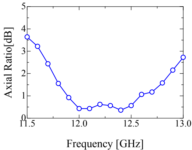
Fig.7. Frequency characteristics of boasight axial ratio for the test RL-MSAA.
