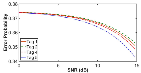
Fig. 2: UWB chipless RFID tags detection's error probability
