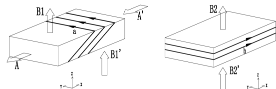
Fig. 1. NFC chip antenna coil configuration of Z-shaped coil (left) and additional coil (right).
