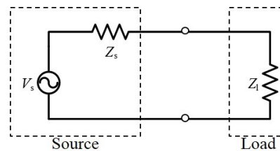
Fig. 1. Generator-load network circuit.
