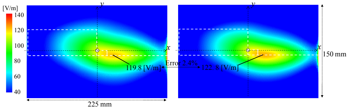
(a) Liquid phantom (b) Solid material Figure 9: Surface electric field distributions at 300 MHz
