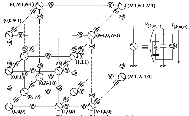
Figure 1: Circuit model.
