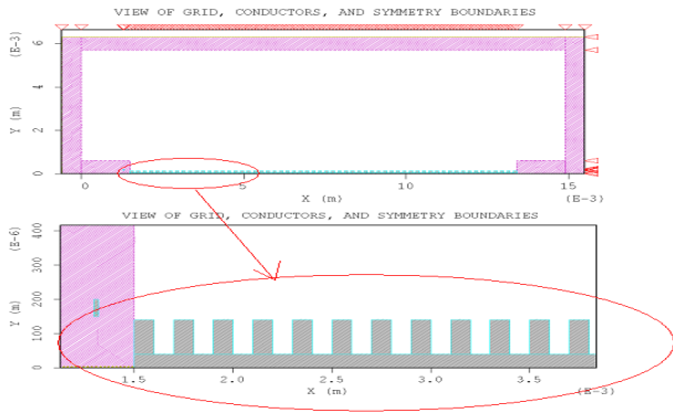
Fig.3 Normal Grating
