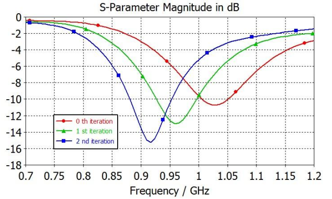
Figure 3: Simulated return loss with fixed length antenna parameter.
