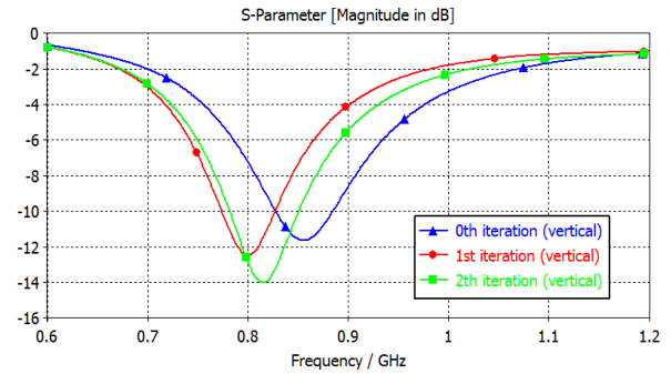
Figure 7: Return loss antenna performance using different iteration with vertical position.
