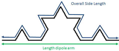
Figure 2: Overall Side Length and Length Dipole Arm
