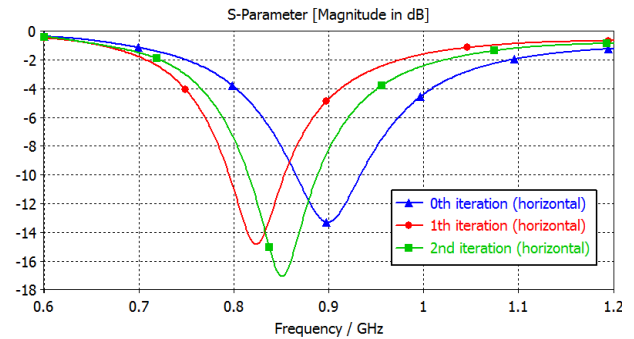
Figure 8: Return loss antenna performance using the different iteration with horizontal position.
