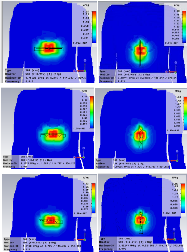
Figure 9: Maximum SAR Value on the human body
