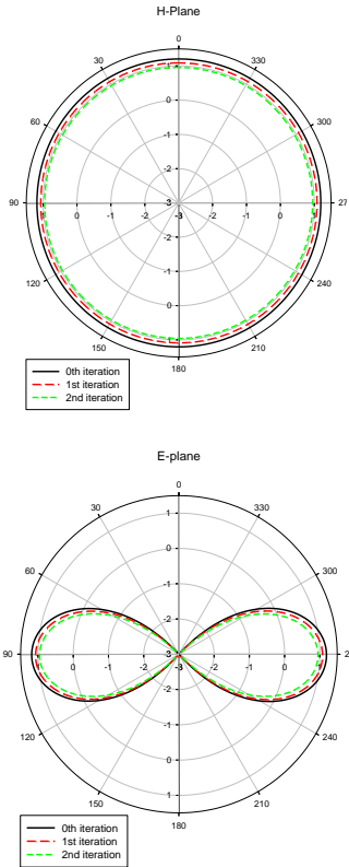
Figure 5: E-plane and H-Plane Radiation Pattern Antenna using Different Iteration
