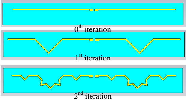
Figure 1 : Antenna design using the first, second and third iteration
