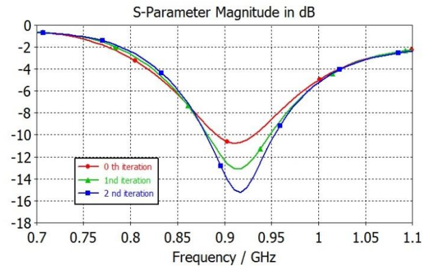
Figure 4: Simulated return loss of optimized at 0.915 GH
