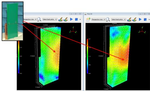
Figure 2. Current distributions on the reference antennas.
