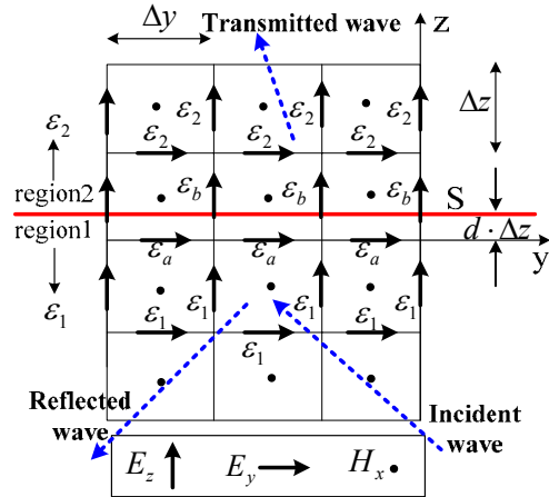
Fig. 3. Example for the effective permittivity calculation
