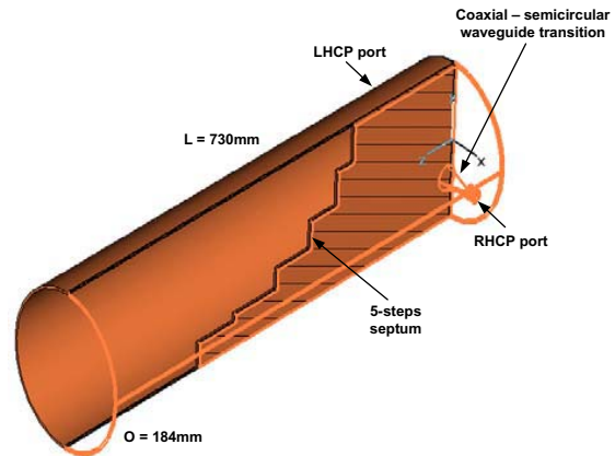
Fig. 15. Proposed septum feed layout
