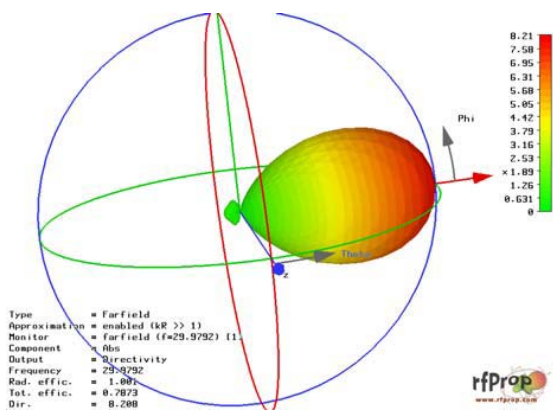
Fig. 12. Radiation pattern of the Yagi-Uda antenna
