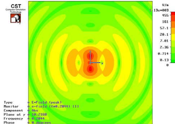
Fig. 1. “Animation” of radiation of the \lambda/2 dipole
