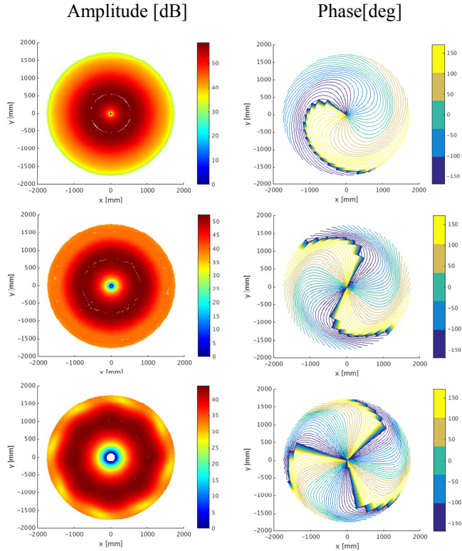
Fig. 2. 2 distribution of a field radiated from our proposed antenna, observed at a distance of 100m ( 50000\lambda_0 ).
