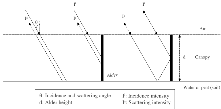
Fig. 4 Schematic diagram of scattering paths considered in the developed model. (a) Direct scattering from ground surface. (b) Direct scattering from alder (wetland forest). (c) Double bounce scattering caused by interaction of alder and ground surface.
