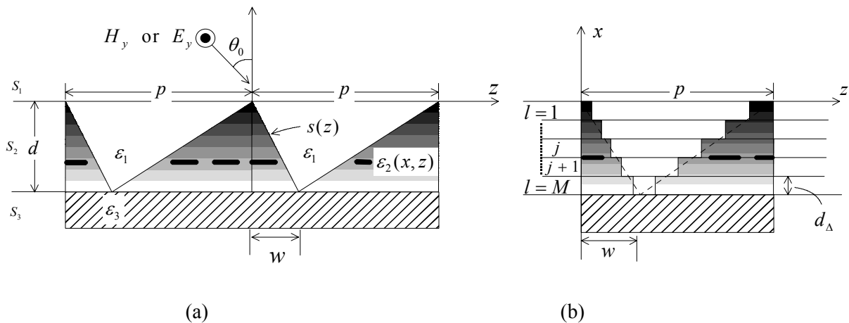
Fig.1 Structure of inhomogeneous dielectric grating with perfectly conducting strip. (a) Coordinate system, (b) Approximated inhomogeneous layers.
