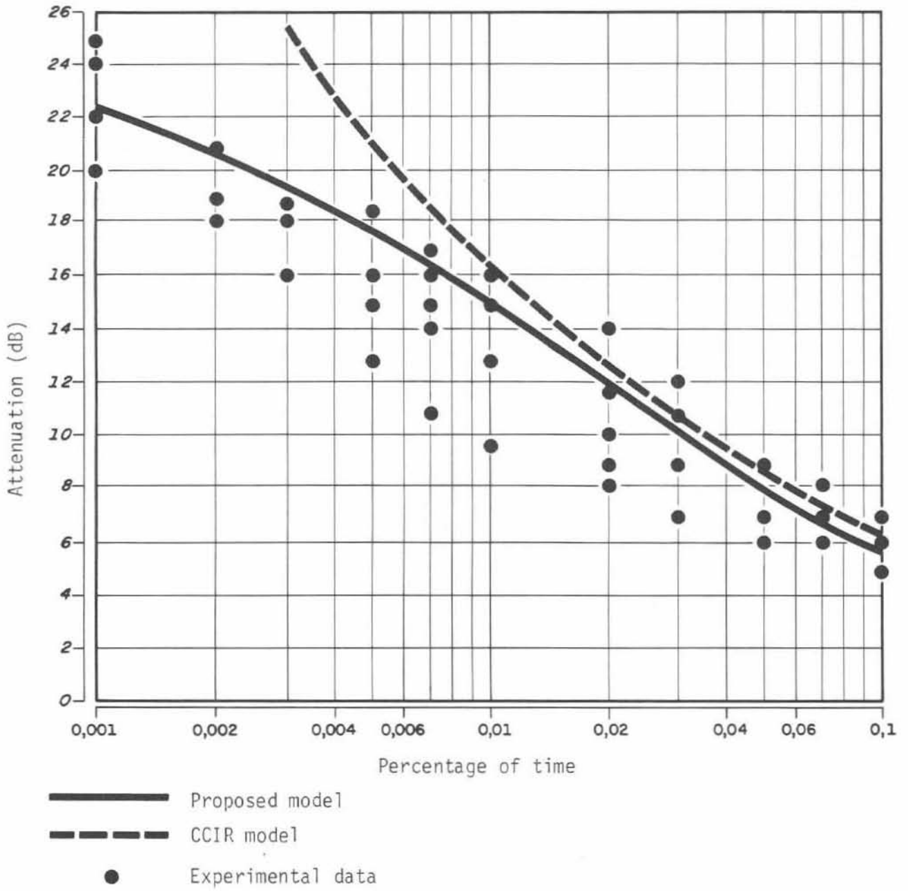
Fig. 1 - Rain attenuation in a terrestrial path - comparison between theoretical and experimental results.
