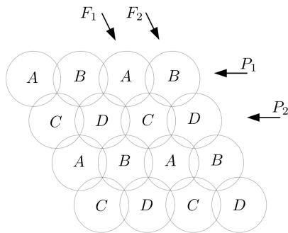
Fig. 2. Beam layout of the 4-color reuse scheme.
