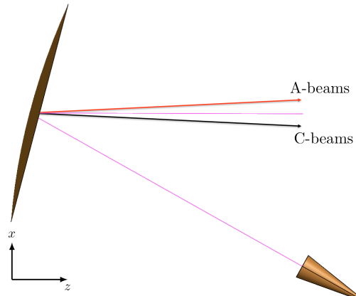
Fig. 3. Curved reflectarray configuration to radiate two types of beams in the 4-color reuse scheme using only a single feed.
