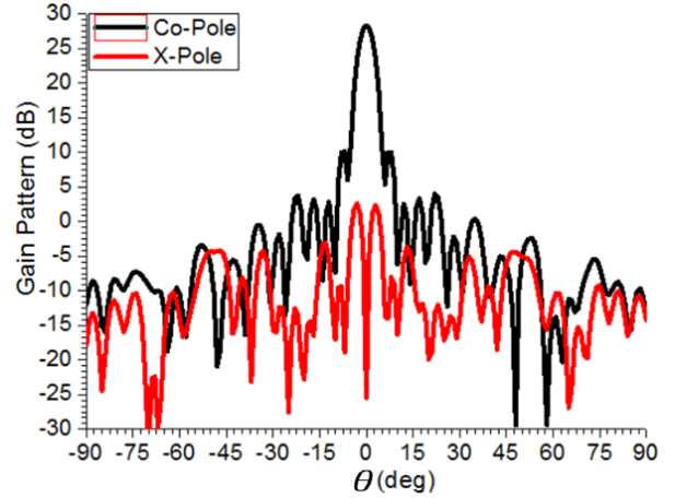
Fig.5. Simulation result of reflectarray antennas at mmW.
