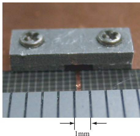
Fig.3 Photograph of the proposed transition
