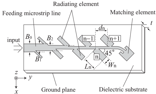
Fig.1 Microstrip comb line array antenna
