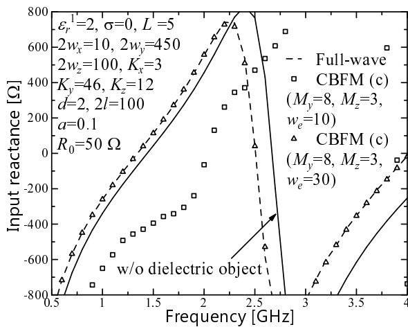
Figure 7: Input reactance: Dipole antenna, (c).
