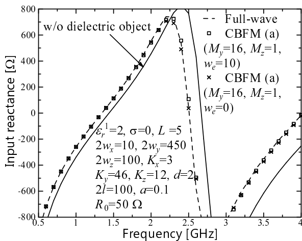
Figure 3: Input reactance: Dipole antenna, (a).
