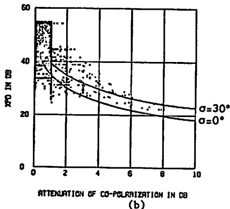
Fig. 6 Cross-polarization discrimination versus co-polar attenuation for the period of August, 1977. Solid lines show the the theoretical results from Oguchi et al. The parameter show the standard deviation of canting angle. (a) 34.5 GHz, (b) 11.5 GHz
