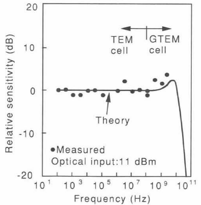
Fig. 5 Frequency response of the Relative sensitivity.
