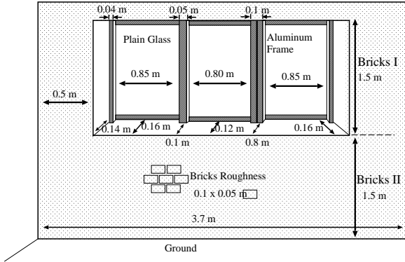
Figure 3: Building surface profile.
