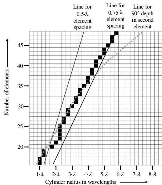
Figure 5. Optimal cylindrical arrays with patch elements. 5 active elements. Black squares show the optimum.
