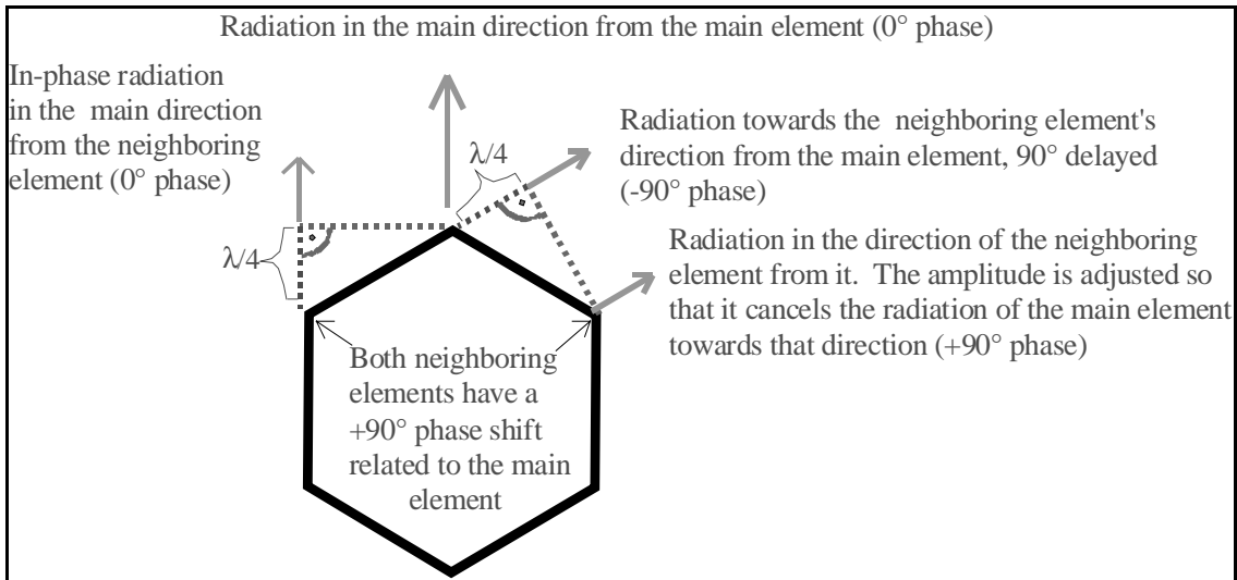
Figure 3. Operation principle of the cylindrical array, making use of array depth
