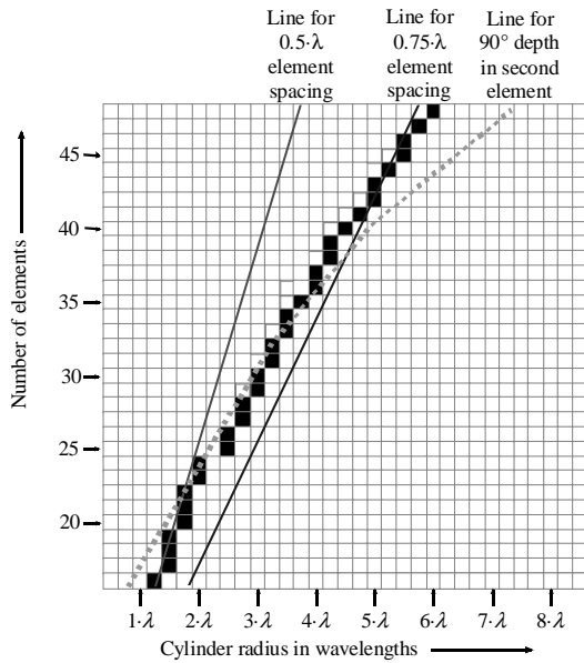
Figure 6. Optimal cylindrical arrays with patch elements. 7 active elements. Black squares show the optimum.
