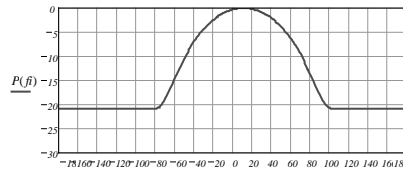
Figure 2. Patch element radiation pattern used in the calculations.
