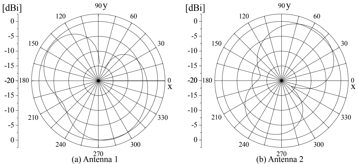
Figure 4: Radiation pattern of two antennas with the slit ( l = 6/50\lambda and d = 8/50\lambda ).
