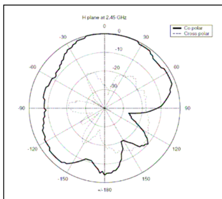
(b)H Plane
