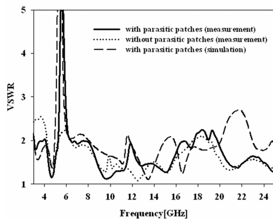
- 959 - Fig. 3. The comparisons of the measured and simulated VSWR values
