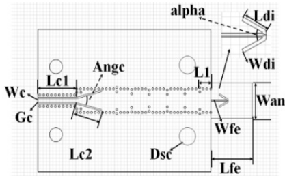
Figure 3. The geometry of filtennas fed by SIW-CPW transition
