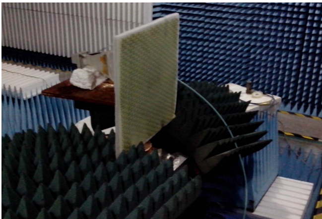
Figure 6 Test environment
