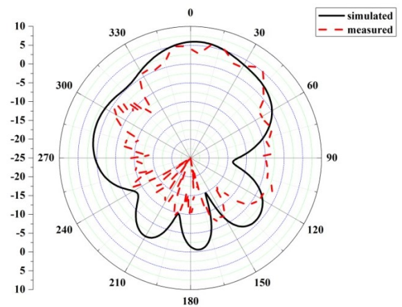
Fig. 9 E-plane radiation pattern at 17GHz
