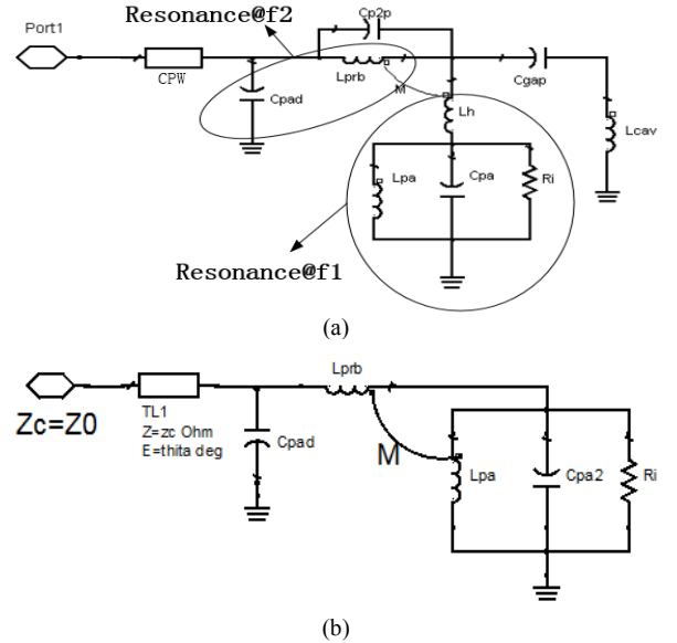
Fig. 4. Circuit model for the proposed antenna. (a) Detailed circuit model, (b) Simplified circuit model: Z_0=75\Omega , C_{pad}=0.166\text{pF} , L_{prb}=0.117\text{nH} , L_{pa}=0.017\text{nH} , M=0.00627\text{nH} , C_{pa2}=0.863\text{pF} , R_i=30\Omega , z_c=234\Omega , \theta_{ita}=194\text{deg} .
