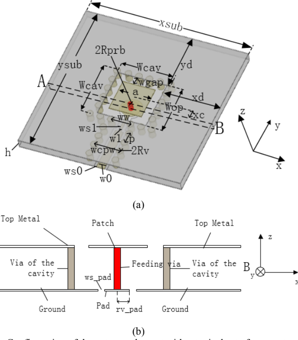
Fig. 1. Configuration of the antenna element with a typical set of parameters: x_{sub}=6.7 , y_{sub}=10 , x_d=0.5 , y_d=3.5 , x_c=0.3 , W_{cav}=3.3 , W_{op}=3 , w_w=1.2 , w_{cpw}=1.6 , w_0=0.5 , w_1=0.15 , w_{s0}=0.15 , w_{s1}=0.2 , w_{s\_pad}=0.15 , w_{gap}=0.5 , r_{v\_pad}=0.53 , r_{prb}=0.15 , a=2 , R_v=0.2 , p=0.65 , all parameters are in "mm". (a) overall view, (b) sectional view.
