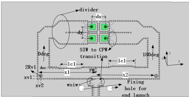
Fig.8. Structure of the 2x2 array. xv1=1.05\text{mm} , xv2=1\text{mm} , dxc=0.36\text{mm} , Rv1=9\text{mm} , lcl=l_{c2}=9\text{mm} , dx=4\text{mm} , dy=3.9\text{mm} , x1=19.57\text{mm} , x2=21.53\text{mm} , wsiw=3.9\text{mm} . The size of the substrate is 64mmx32mm.
