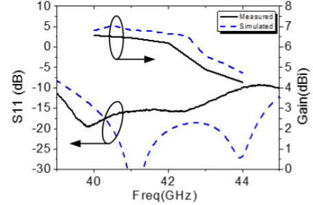
(a) Return loss and boresight Gain
