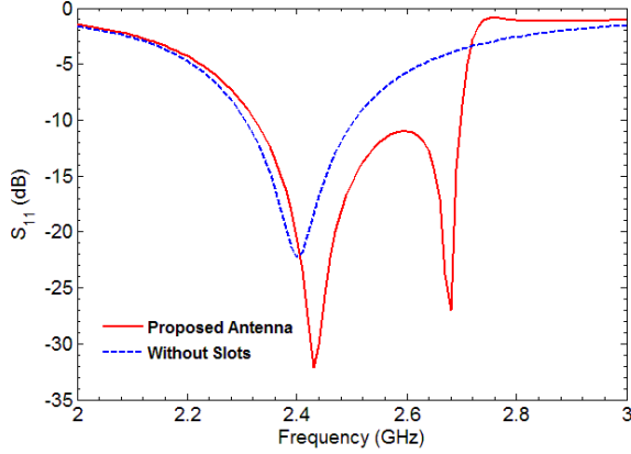
Figure 2. Reflection coefficients of the proposed antenna and without slots
