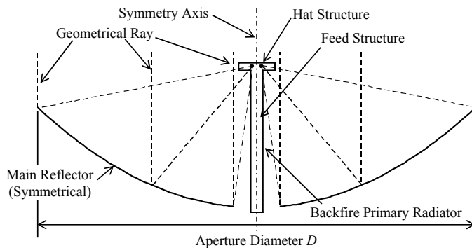
Figure1. Antenna Structure
